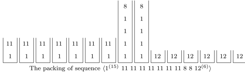
Figure 1 The optimal packings for two sequences of the family when n = 30 and m = 6 (item sizes and bin capacities are scaled by 2m = 12 ).
