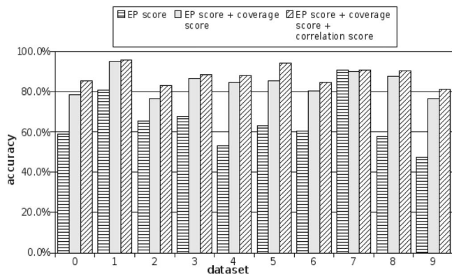
Fig. 6. Analysis of the score function.
