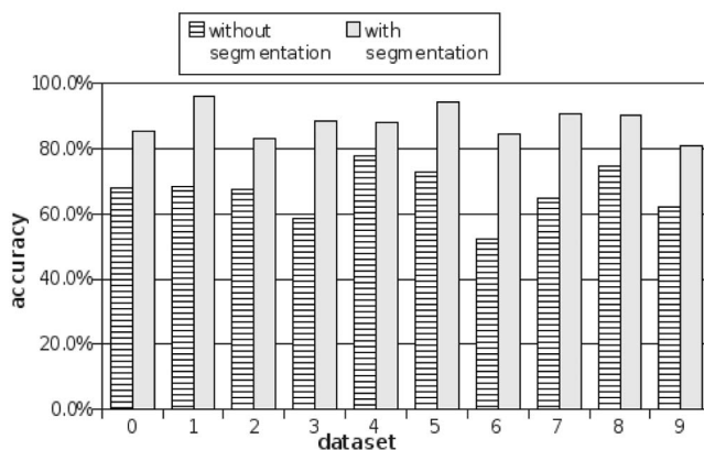
Fig. 7. Effect of the trace segmentation algorithm.
