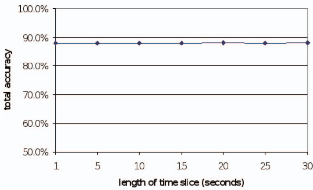
Fig. 8. Effect of the time-slice length \Delta t .
