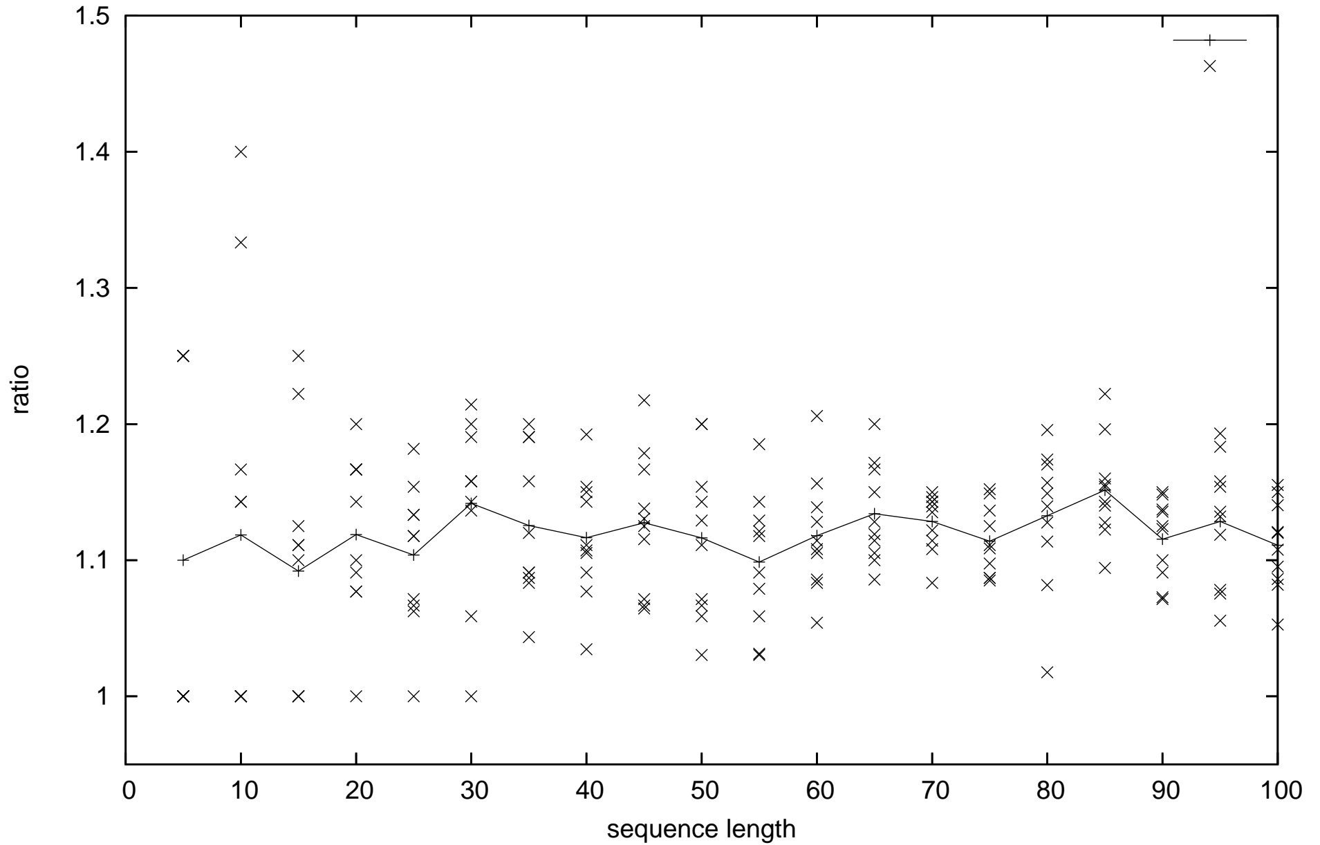
Classic Bin Packing, uniform data, comparing NextFit to WorstFit, sample size 10
