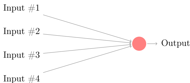
Figure 1: A Perceptron.
